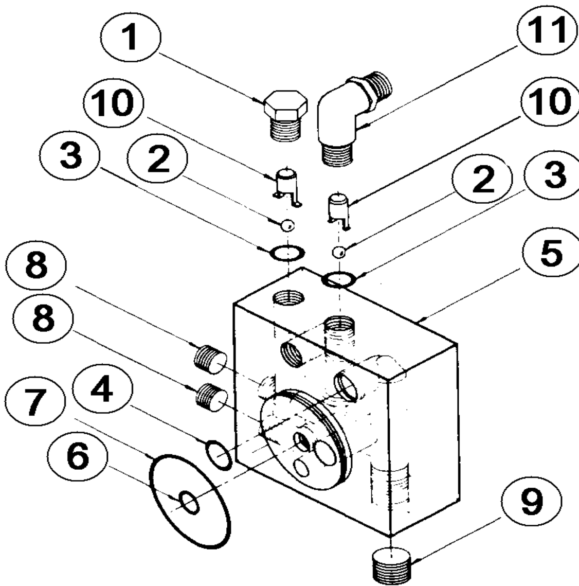
Figure 14. Head Assembly
